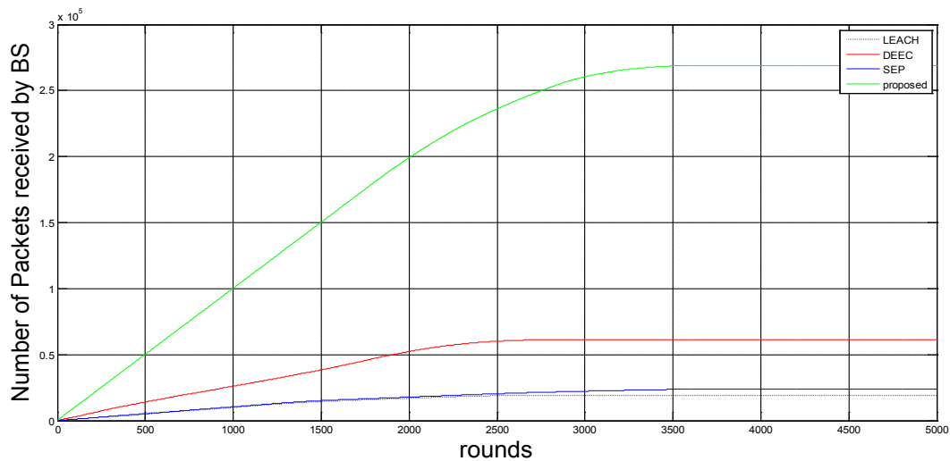
Figure 9: Throughput.
