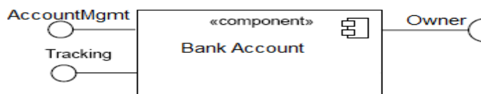
Figure- 1. A UML Component with two provided and one required interfaces.
